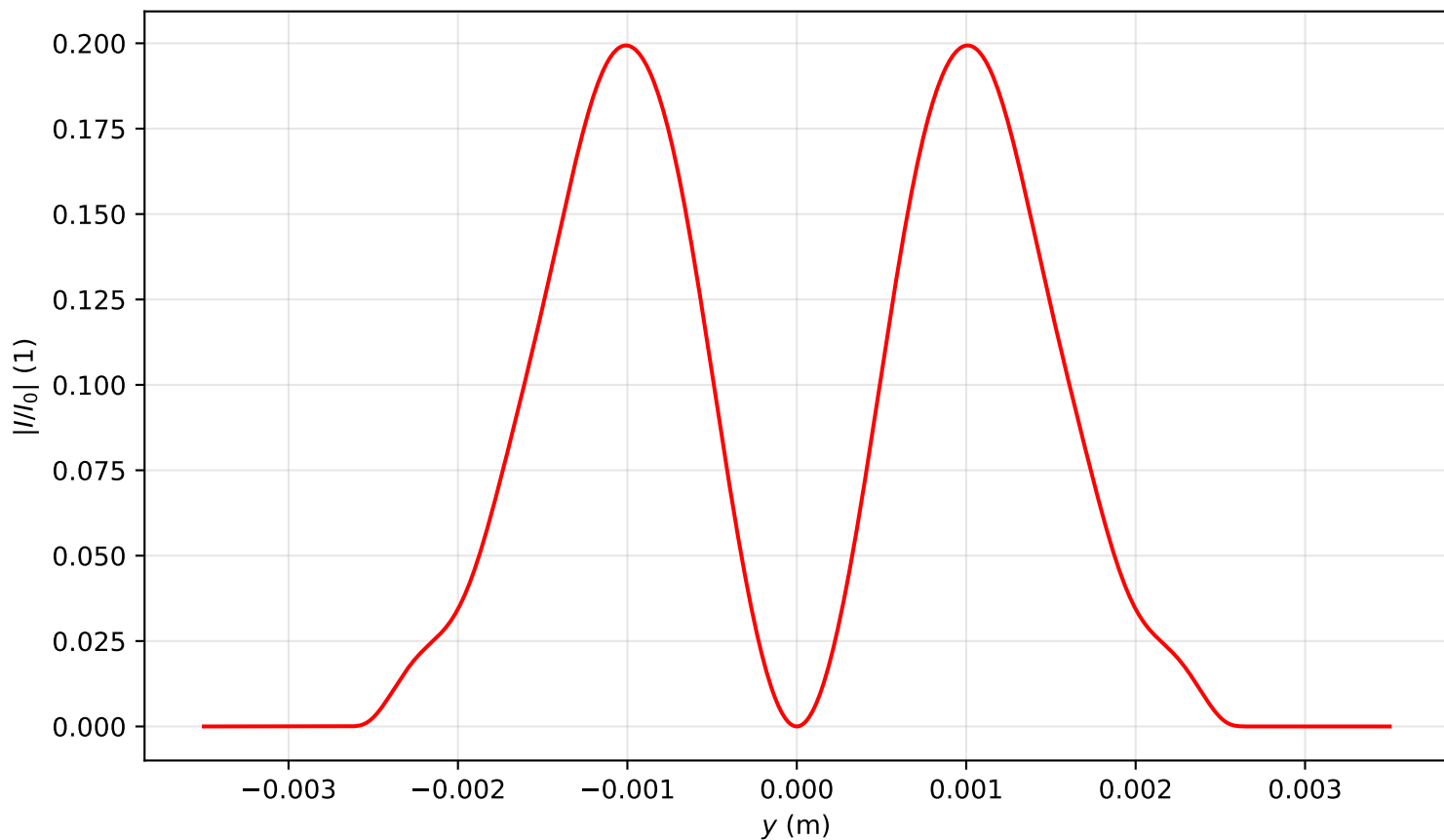
Intensity profile I(x=0, y, z=3.582)/I_0 , \text{Pin}=0.5\text{Pcr} , artificial time
